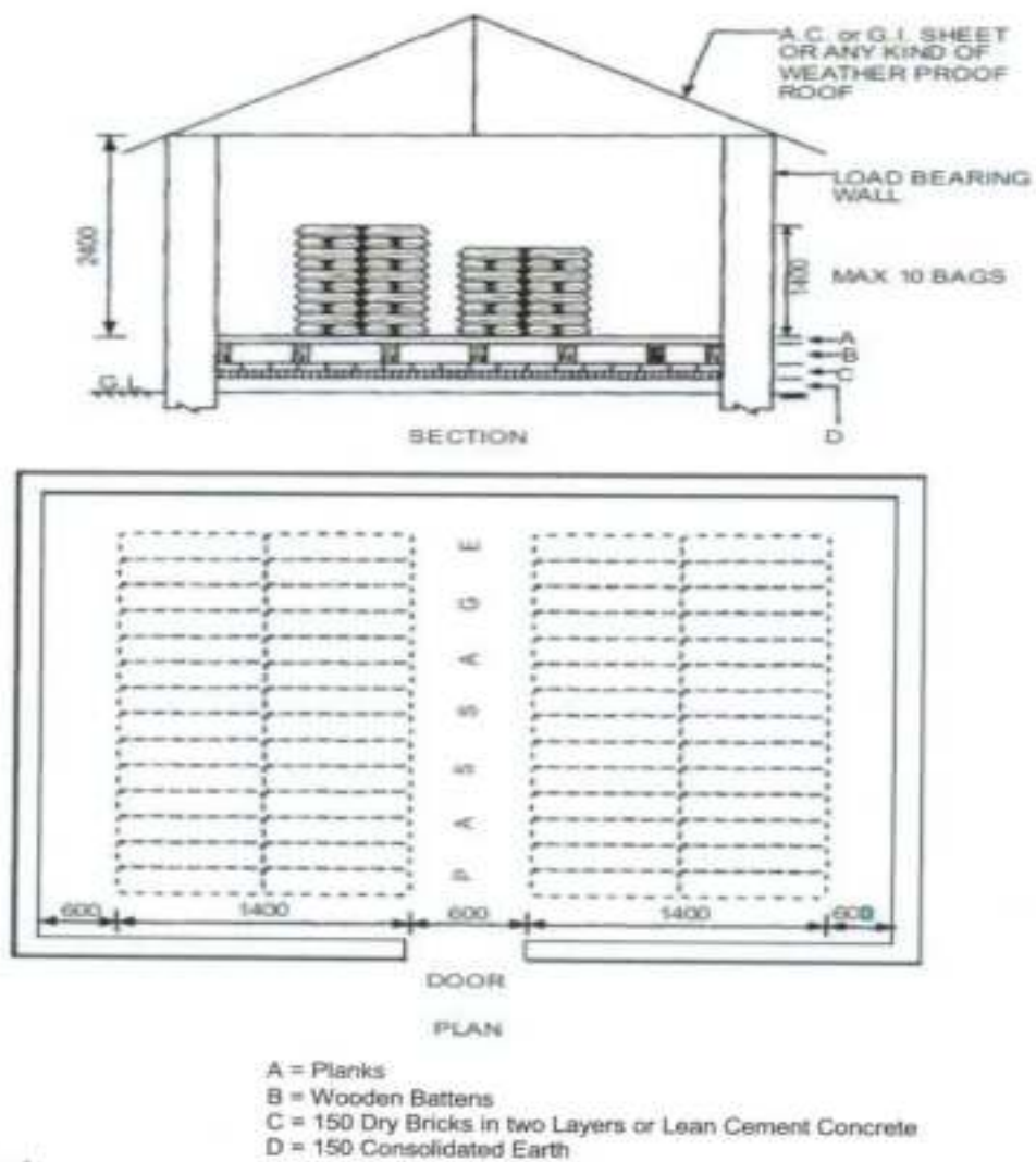
Fig. 1.1 : Typical Arrangement in Cement Godown
